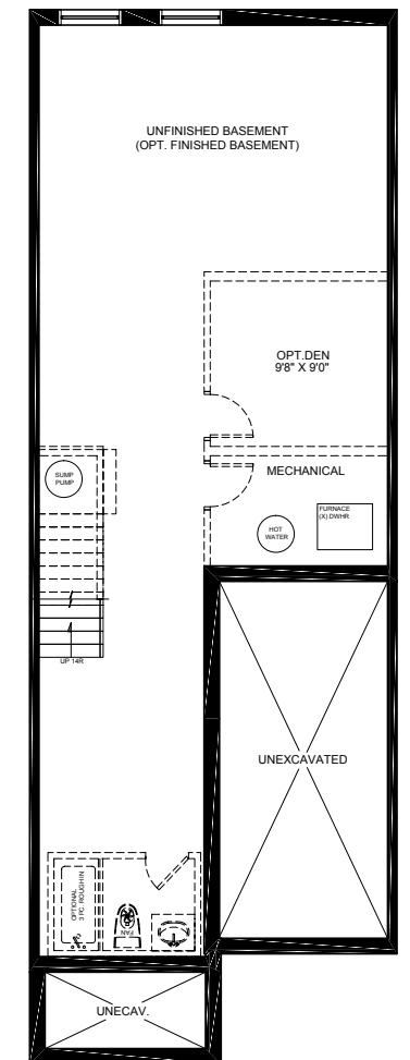
Basement Modern & Country (Blocks 3 & 4)
