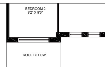
Second Floor Country Alt (4 Bedrooms)
