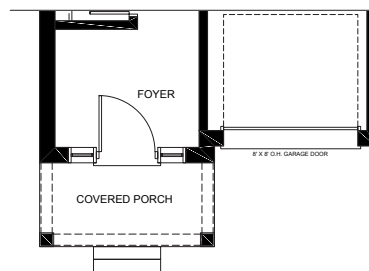
Ground Floor Country
