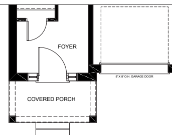
Ground Floor Country
