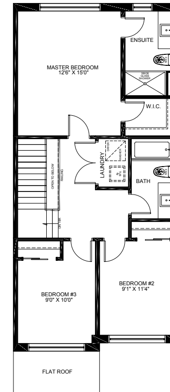
Second Floor Modern
